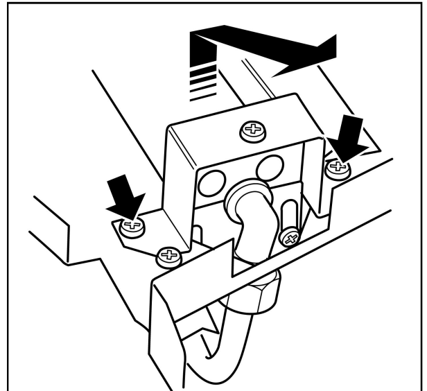
Figure 52. Removal of burner
