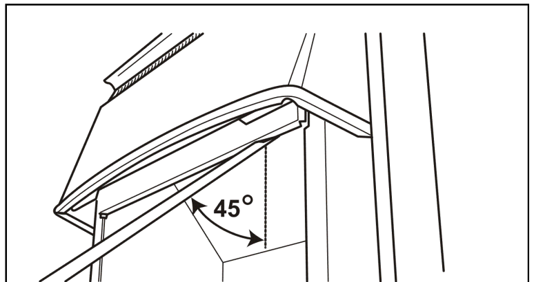
Figure 37. Spillage check
